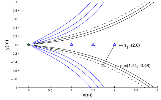
Fig. 4. Examples of the contours described by Equation (14) and (15) for a target at (0,0) (shown as a star), r_1 \in \{1, 1.5, 2\} and \lambda_d set to .01 (black lines of lesser curvature) or .05 (blue). \sigma_s was 1 and N_1 was 1. For example, if the robot first travels to the position s_1 = (2,0) and takes one measurement then it can take all remaining measurements from anywhere on the dashed curve (e.g., s_2 as labelled) to satisfy \underline{\lambda}(\mathbb{F}) = \lambda_d .
