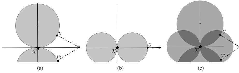
Fig. 7. An illustration of the constraints on the measurement sequences. (a) by Equation 6, (b) by Equation 7, and (c), the intersection. Note the radius in (b) is never greater than the radius in (a). Assuming the other measurements are placed, the last measurement U , must fall in the regions specified, while traveling the least. The dotted line adjoining U and the starting location illustrates the shortest path.
