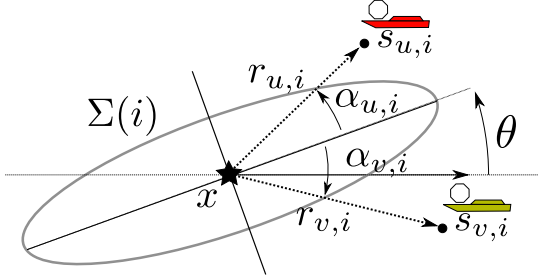
Fig. 2. The target-local coordinate frame. By expressing the measurement locations (black dots) with respect to the frame rotated by \theta , \mathbb{F} is a diagonal matrix. The covariance ellipse's eigenvectors are aligned with the frame in which we express sensor locations.
