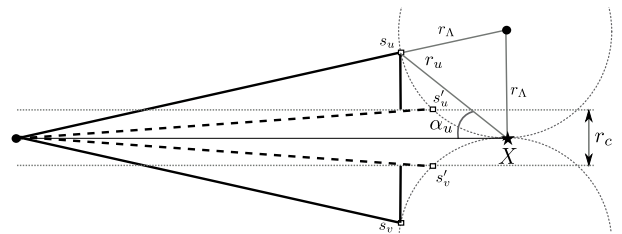
Fig. 9. An illustration of two different choices for communication-constrained measurement locations. s_u and s_v represent the output of Algorithm 2. From these locations, the robots can move directly toward each other to communicate. Alternatively, they can move to s'_u and s'_v , and remain in communication during measurement. Algorithm 3 finds the optimal placement of symmetric measurements to minimize the cost while including the rendezvous cost.
