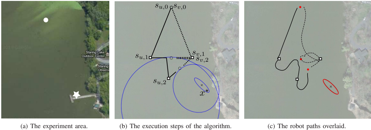
Fig. 11. Experiment results from Lake Staring, Minnesota, USA. (a) : The experiment area. The true target (and camera in [29]) were placed on the docks near the bottom right corner (labelled with a star). The robots began near the top-middle (circle). (b) : The two calls to Algorithm 3 produced the dark paths shown, and reduced the uncertainty (the blue circles). The final actual uncertainty was the solid ellipse. (c) : More execution details. The solid red circles are the points where the robots exchanged information. The figure covers an area approximately 200m vertically by 150m horizontally.
