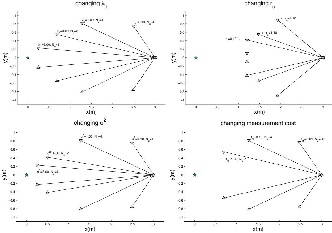
Fig. 8. Optimal two-robot trajectories for various system parameters. In all figures the robots started at location (3, 0) and the true target was at (0, 0) . Communication constraints were only considered in the top right figure and all other parameters were held fixed. Top-left: \lambda_d \in \{.1, 1, 3, 8\} . Top-right: r_c \in \{2.1, 1.1, .1\} . When r_c = .1 , the robots rendezvous after measuring. When r_c = 2.1 the output is the same as the result from unbounded r_c . Bottom-right: t_m \in \{.01, .1, 1\} Note that as t_m increases, the optimal algorithm travels to more informative locations so that fewer measurements are required. Bottom-left: \sigma \in \{.1, 1, 4, 8\} . Note that changing the sensor noise produces the same effect as requiring more information (compare left two figures).
