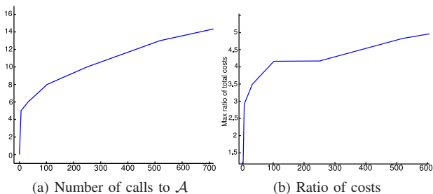
Fig. 12. The aggregate results of numerical studies. Left: the number of calls to \mathcal{A} as a function of \frac{\lambda_d}{\lambda_{F_0}} . Right: the ratio of costs of online algorithm to optimal offline algorithm, as a function of \frac{\lambda_d}{\lambda_{F_0}} . Shown is the maximum value encountered during simulations.
