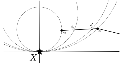
Fig. 3. An illustration of Lemma 2. Three or more measurement locations are sub-optimal in the case of a single robot. Two measurement locations s_1 and s_2 can be moved closer together to produce a lesser-cost trajectory with the same information. This process can be repeated until the pair of measurement locations is collapsed to the same point.
