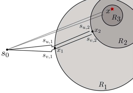
Fig. 10. An illustration of the two-robot MULTI-STEP algorithm (solid paths) and the optimal \mathcal{A} algorithm (dashed paths). The robots begin at location s_0 . The optimal choice is to move directly to x^* , but we are unsure of the location of x^* . Thus, we form a convex region R such that the probability x^* is in R is high. At each step of the MULTI-STEP algorithm, we do less work than \mathcal{A}(s_0, x^*) by Lemma 5. Since the number of \mathcal{A} executions is bounded by Lemma 6, we do not do significantly more work than optimal by Theorem 3.
