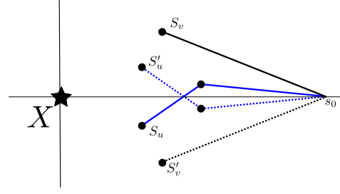
Fig. 6. The steps of the proof of Lemma 4. First, the optimal two-robot strategy, S^* = \{S_u + S_v\} , is “mirrored” about the line \overline{x^* s_0} . Since the information from the two pairs of symmetric strategies, S'_u + S_u or S'_v + S_v , is twice the required information, it is clear that one of the two pairs produces the required information.
